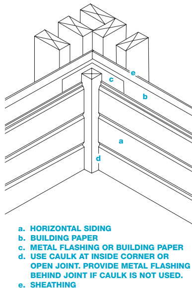
Inside Corner Detail-b
