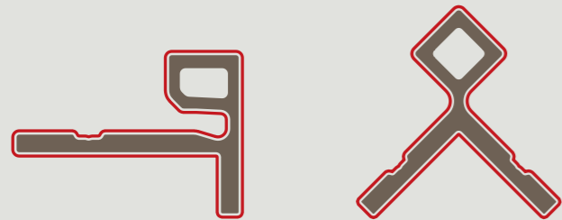
F Trim UH50 3.0 x 2.1 in
